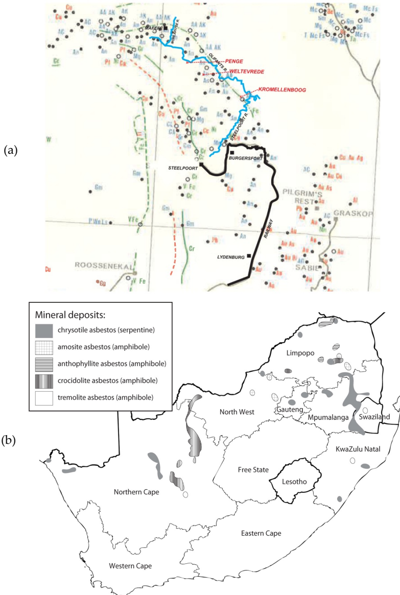
Figure 4. a. Map of the mineral deposits in the Transvaal Crocidolite-Amosite (Pietersburg) asbestos field located on the north-eastern border of the Bushveld Igneous Complex. b. Map of South Africa showing
